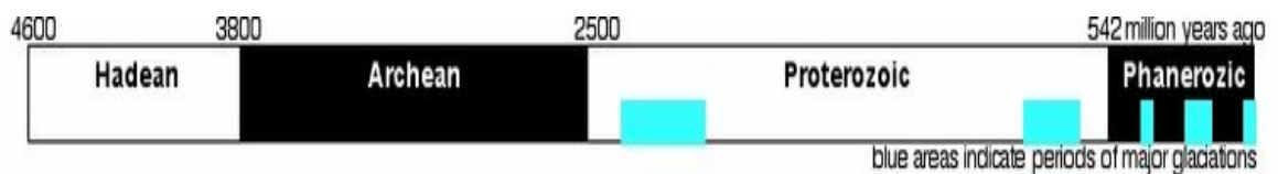
Figure 30. Major glacial periods in earth's history. www.en.Wikipedia.org/wiki/Timeline_of_glaciation .
