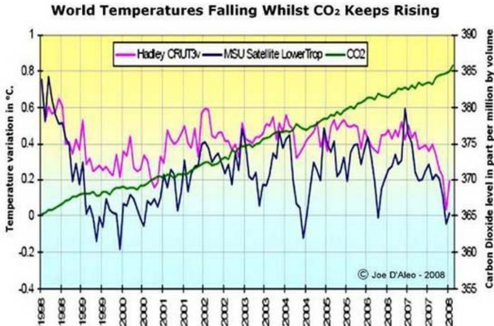
Figure 21. World temperature is falling while atmospheric CO 2 is rising. Data for a) Average Mean Temperature of Earth's Surface: UK's Hadley Climate Research Unit CRUT3. b) Lower Troposphere Temperature Measurements: NASA's Microwave Sounding Unit (MSU). c) Atmospheric CO 2 concentration: Mauna Loa Observatory, Hawaii, USA. http://icecap.us/images/uploads/Correlation Last Decade pdf
