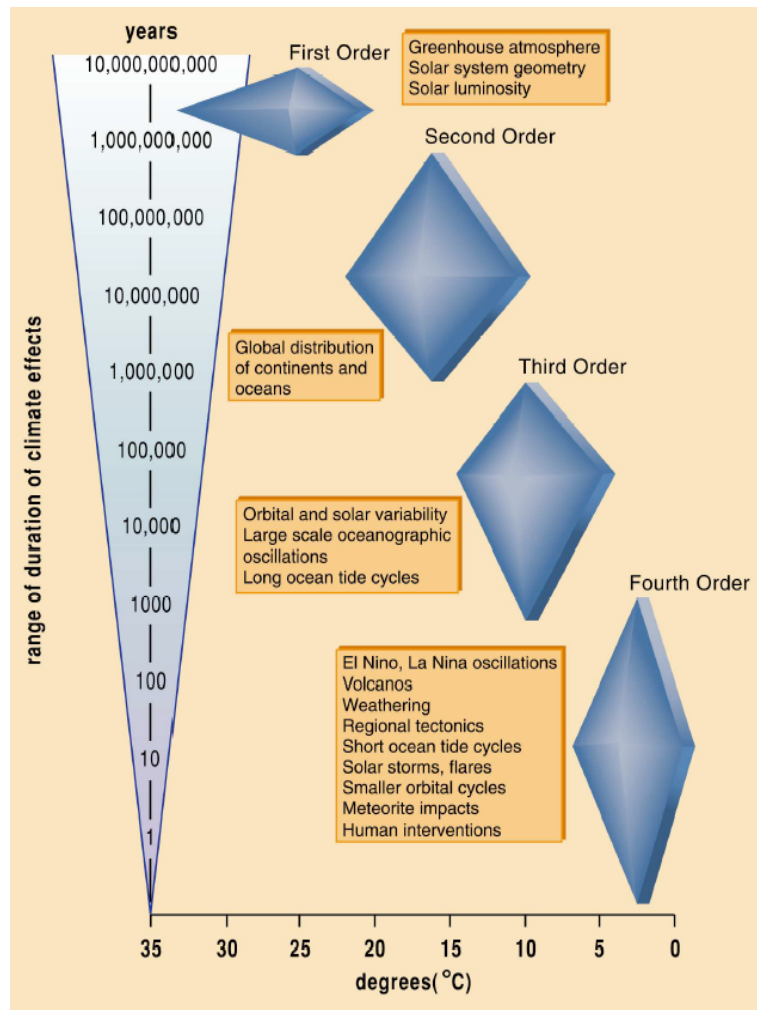
Figure 29. Geologic constraints on global climate variability. Natural climate drivers ranked by intensity and duration. Human interventions meteorite impacts, volcanic eruptions, El Nino and others are considered the 4 th Order affecting climatic variability, Gerhard, 2004
