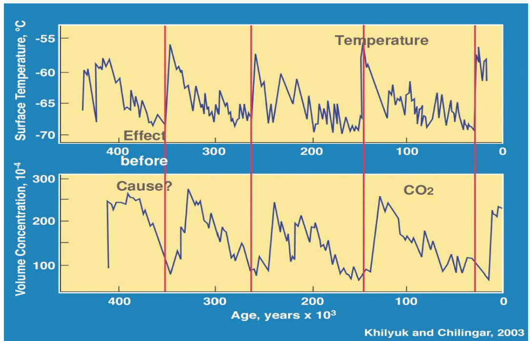
Figure 19. Time lag between maximum temperatures and atmospheric CO 2 concentration during the Quaternary, Khilyuk and Chilingar, 2003.
