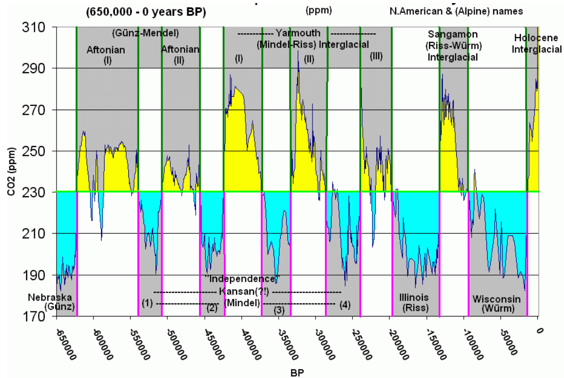
Figure 2. Late Pleistocene Epoch: Atmospheric CO 2 and the Glacial Cycles. Time Line Glaciations, 2009. Pleistocene Climate Cycles. www.en.wikipedia.org/wiki/Timeline_of_glaciation .
