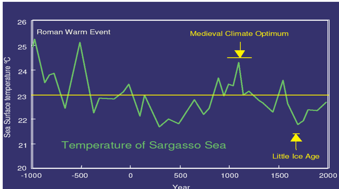
Figure 6. Sea surface temperatures from the Sargasso sea during the last 3000 years based on oxygen isotopic ratios of Globigerinoids rubber (Plankton) collected from a box core through 50 cm of bottom sediment, Keigwin, 1996
