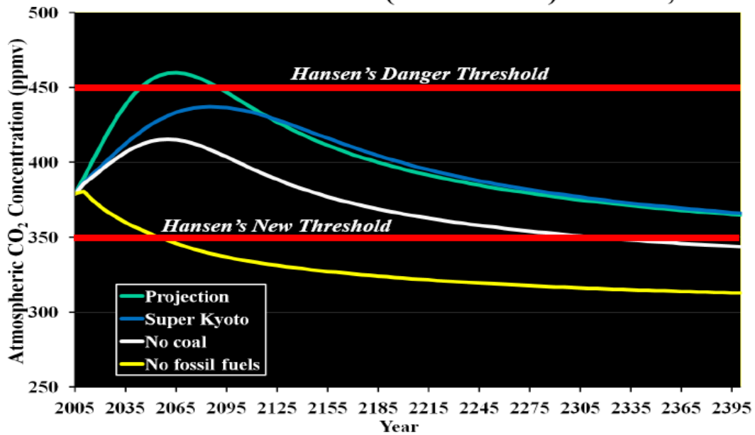
Figure 22. Atmospheric CO 2 concentrations with various carbon emission scenarios from 2005 AD to 2400 AD, Caltech 2008. Data from rutledge.caltech.edu, October 2008. ( Copyright, Hughes, 2009) Worth noticing is the background of 325 ppmv atmospheric CO 2 concentration without the use of hydrocarbons, the same as Beck 2007 and the same if all Calendar's, 1985,data are taken into account
