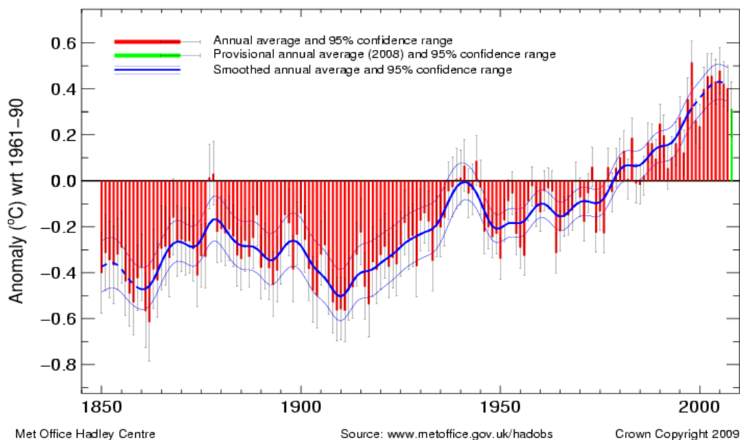
Figure 9. Global temperature record 1850-2008, Jones, 2008, and http://hadobs.metoffice.com/hadcrut3/diagnostics/global/nh+sh/
