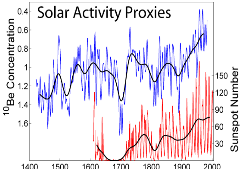
Figure 28. Solar proxy activities based upon 10 Be concentration found in Dye-3, Greenland ice core. Beer et. al., 1994. 10 Be originates from the incoming galactic dust. Relation to Sunspot number from 1600 AD to 2000 AD, Hoyt and Schatten 1998a, 1998b
