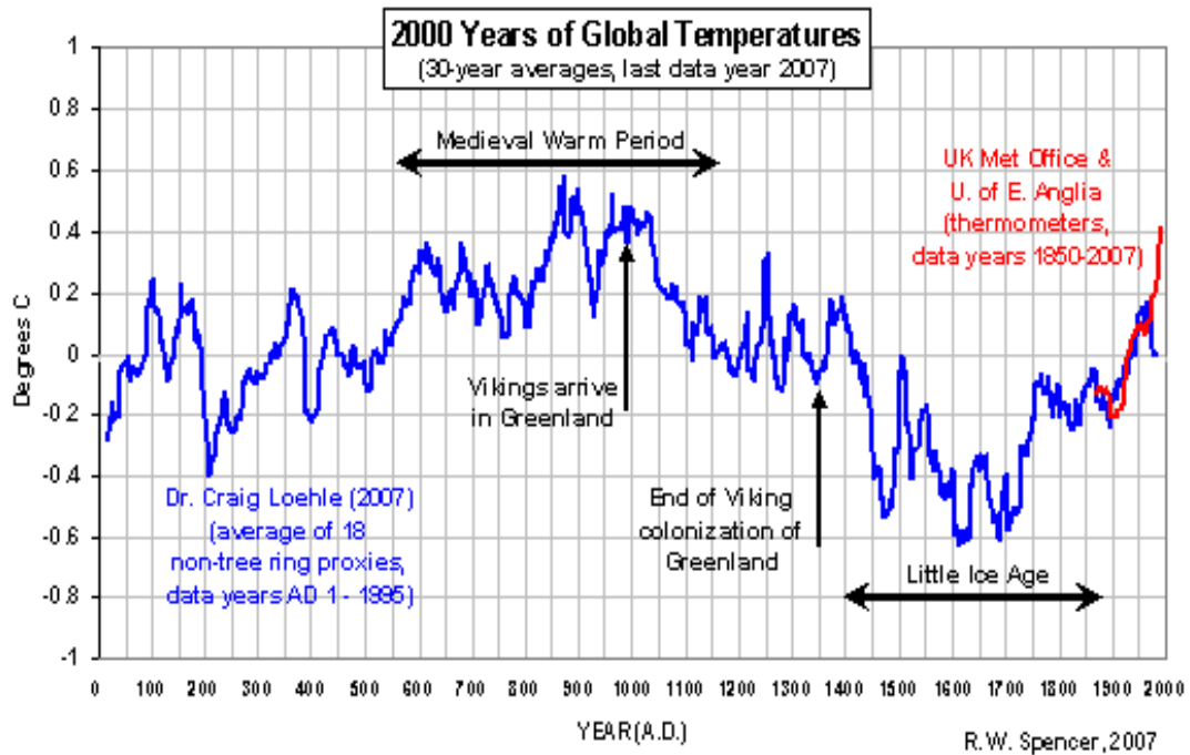
Figure 7. 2000 years of global temperatures based upon 30 year averages, Spencer, 2007.
