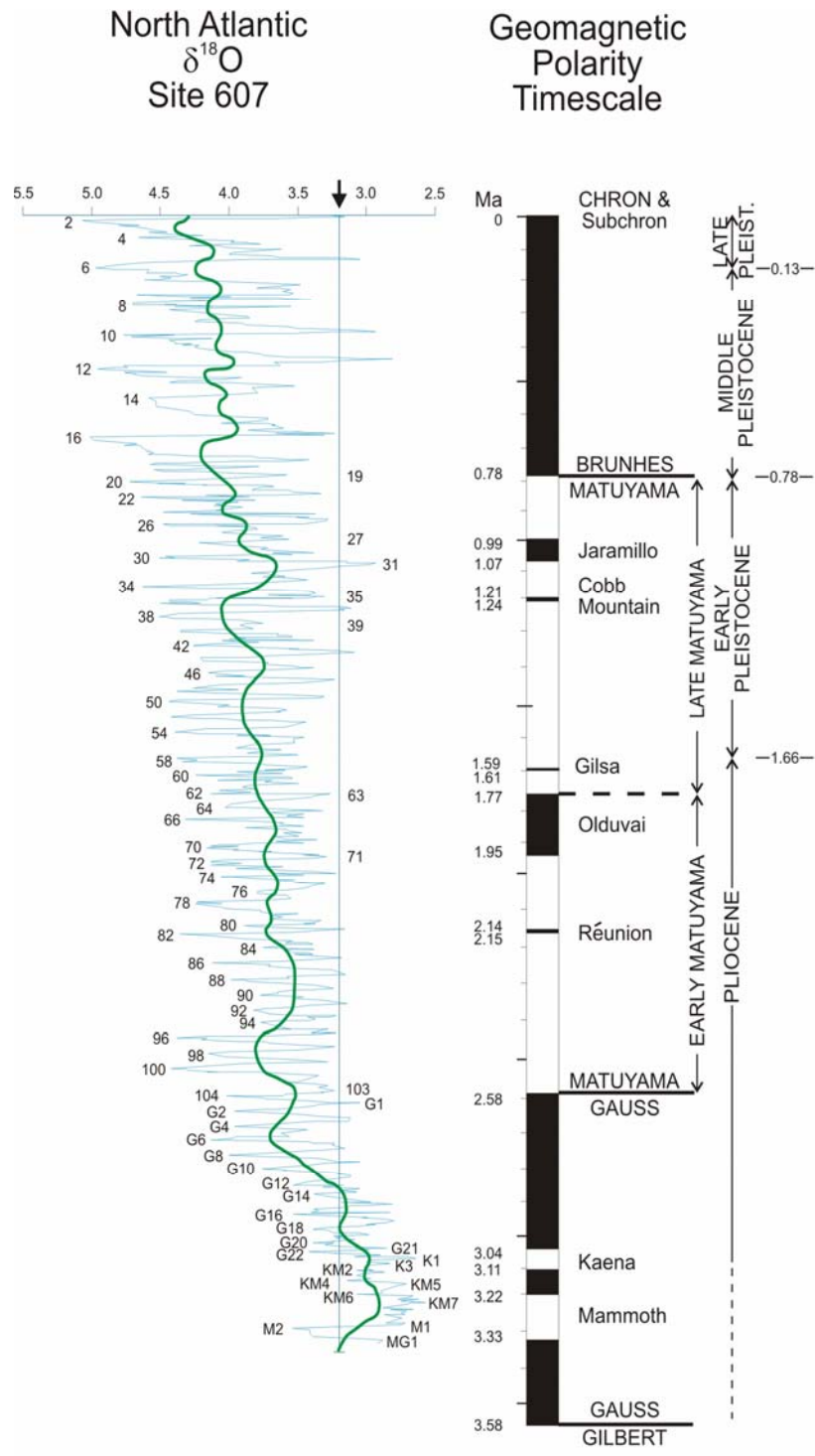
Figure 4. Geomagnetic polarity scale (Candle and Kent 1995) and \delta^{18}\text{O} paleotemperatures record from site 607 in the North Atlantic (Ruddiman et.al., 1989; Raymo 1992)
