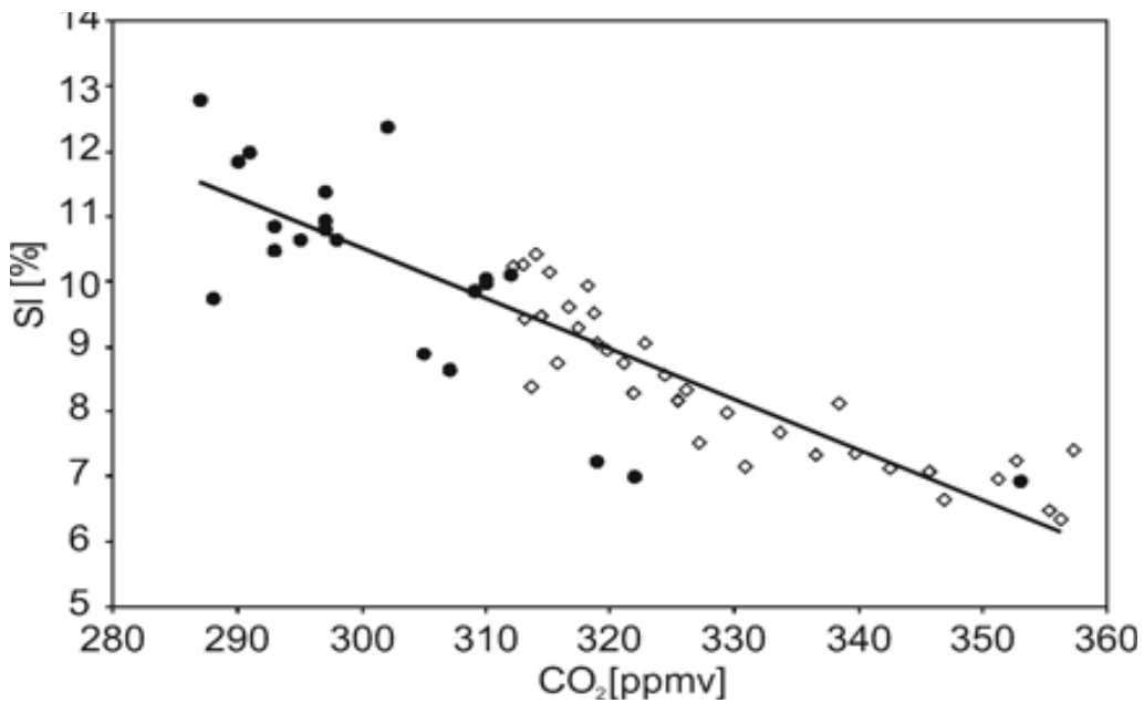
Figure 11. Correlation of stomata frequency ( stomata index=SI) to atmospheric CO 2 from fossil leaves of B. Pendula (black circles) and P. Pubescens ( white circles) in lake Little Grisbe, Danemark, Wagner et. al, 2004.
