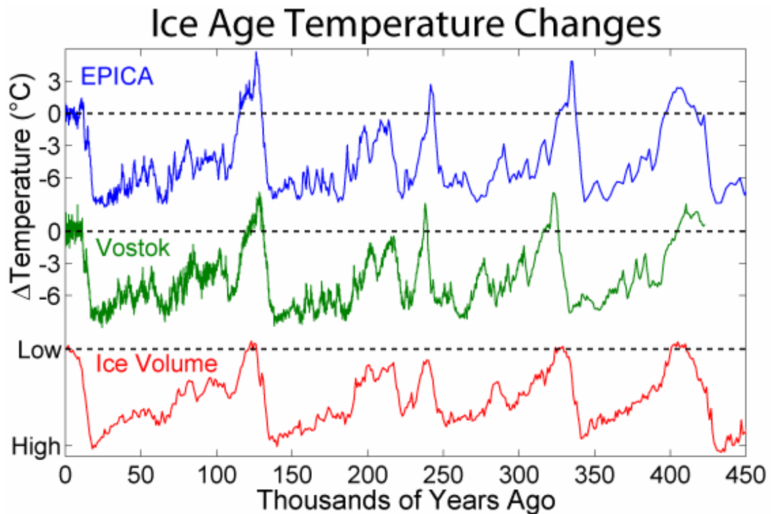
Figure 3. Climatic changes as documented from Vostok-1 icecore data, Petit et. al., 1999, and EPICA icecore data, EPICA, 2004, for the last 450,000 years. Worth noticing is the rise of temperature well above the today's one during the long interglacial periods without the complete melting of the ice caps
