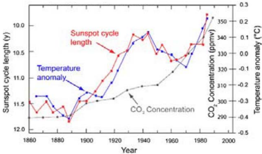
Figure 20. Correlation between sunspot cycle length, temperature anomalies and atmospheric CO 2 concentration, Friss-Christiensen and Lassen , 1991
