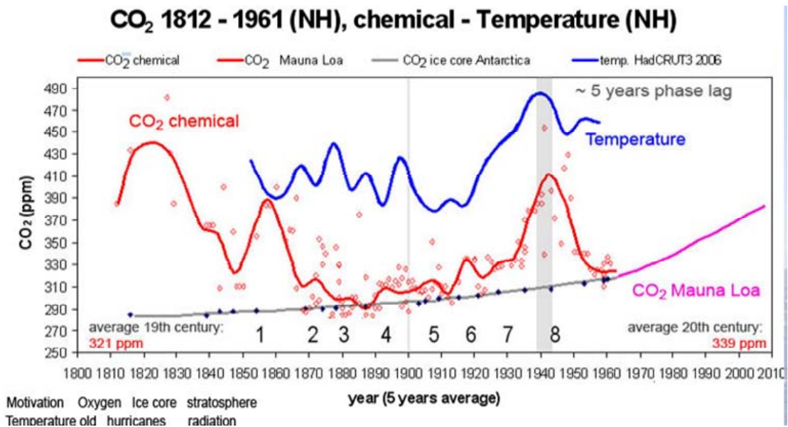
Figure 1. Evidence of variability of atmospheric CO 2 concentration during the 20 th century in the Northern Hemisphere Beck, 2007.
