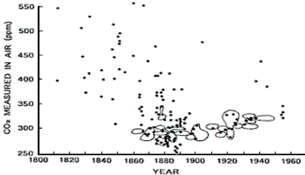
Figure 14. Average atmospheric CO 2 concentrations measured in the 19 th and 20 th centuries, Calendar 1958. Calendar rejected both higher and lower values to arrive at the desired background CO 2 value of 290 ppmv. If he had considered all CO 2 values the concentrations would have been 320 ppmv for the 19 th century, Jaworowski et. al., 1992, Slocum, 1995.
