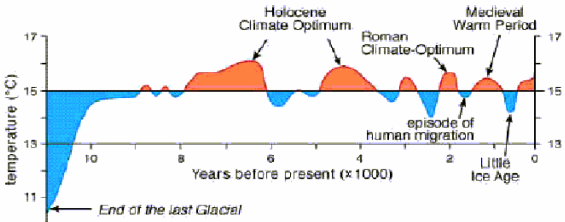
Figure 5. Average near surface temperatures of the northern hemisphere during the past 11000 years Dansgaard et al., 1969 & Schonwiese 1995.
