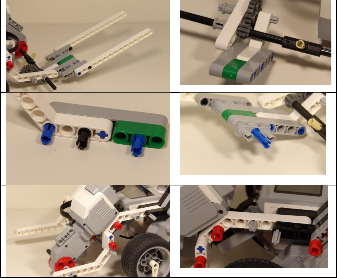
Forklift Mechanism
