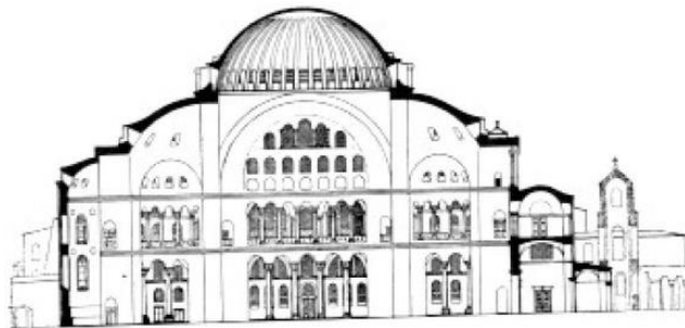
66 Sancta Sophia, Istanbul. Section after A. M. Schneider
