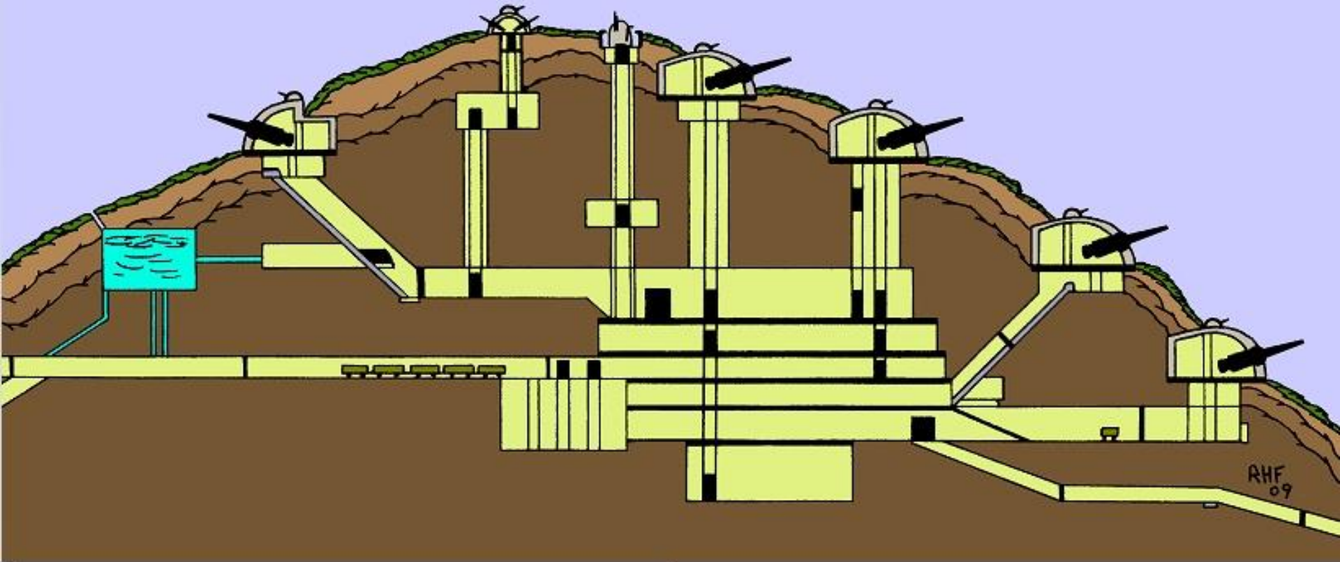
Maginot Line Fortification Cross-Section
