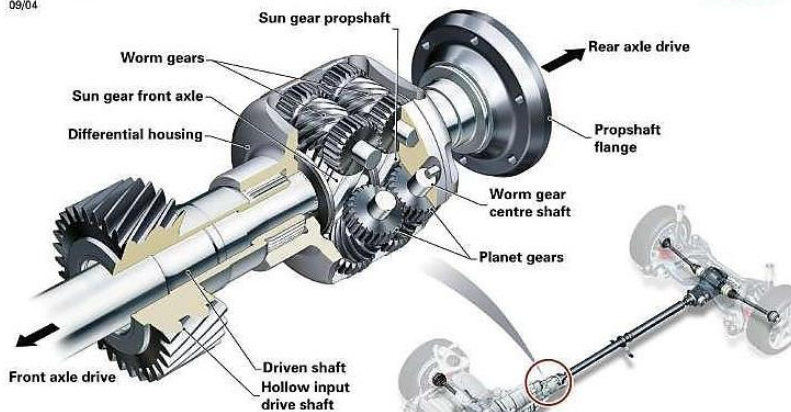
Audi A4 quattro Torsen Differential 09/04
